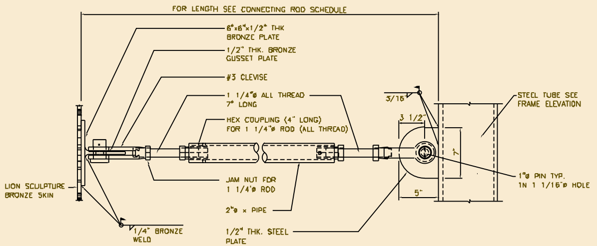
TYPICAL CONNECTING ROD DETAIL A
