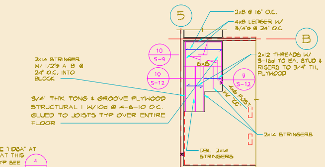
TYPICAL ENTRY FRAMING PLAN A SCALE 1/8"=1'-0"
