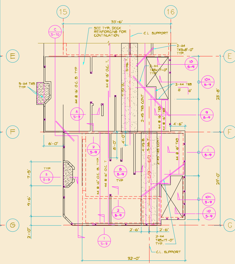
CONC. DECK INNER REINFORCING PLAN BUILDING H SCALE 1/8"=1'-0"
